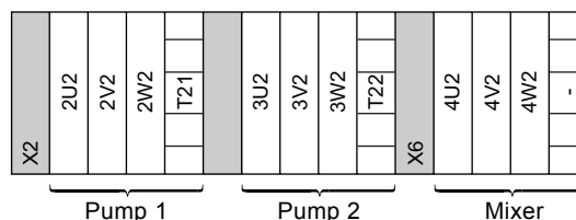
Fig. 4 Terminal blocks X2 and X6, mains supply
