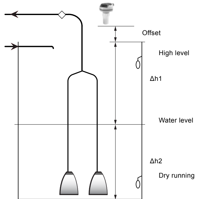
Fig. 14 Ultrasonic sensor
