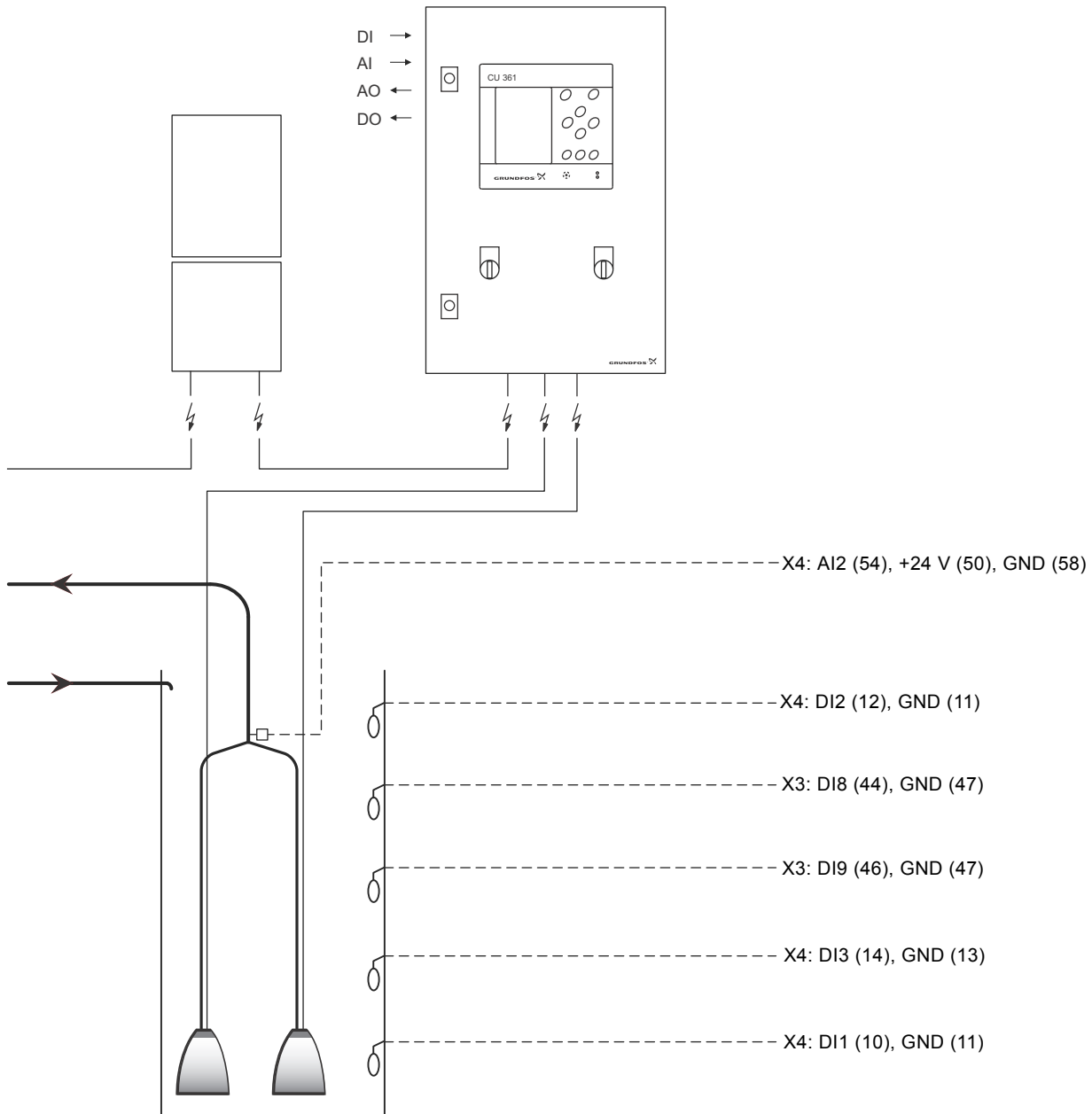
Fig. 9 Two pumps with five float switches
