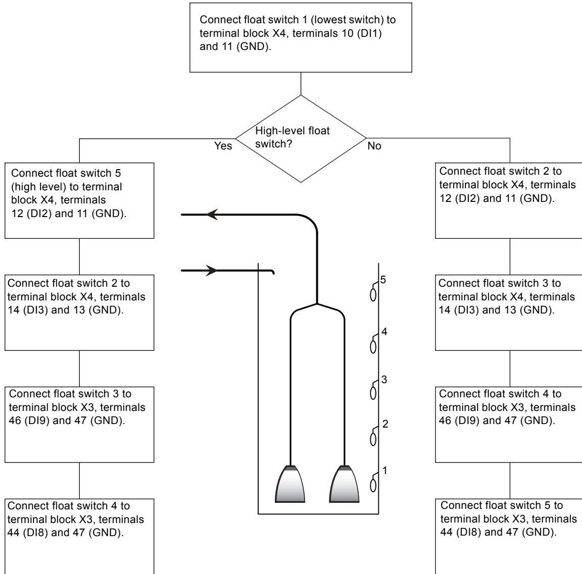
Fig. 12 Float switch installation
