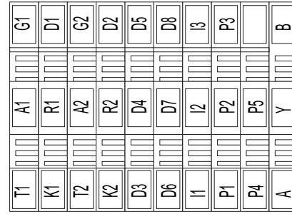
Fig. 7 Terminal block X7, IO 111
