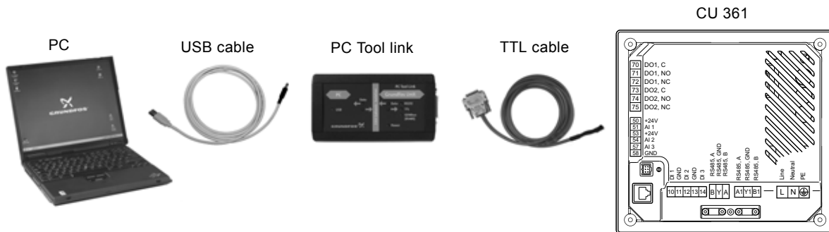
Fig. 18 Configuration by PC Tools
