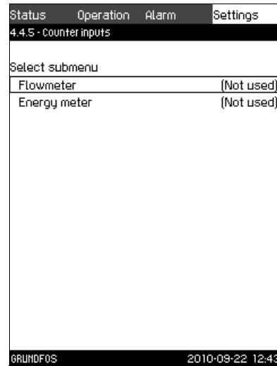
Fig. 32 Counter inputs
