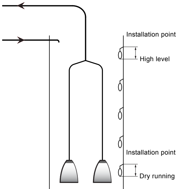
Fig. 11 High-level and dry-running float switches
