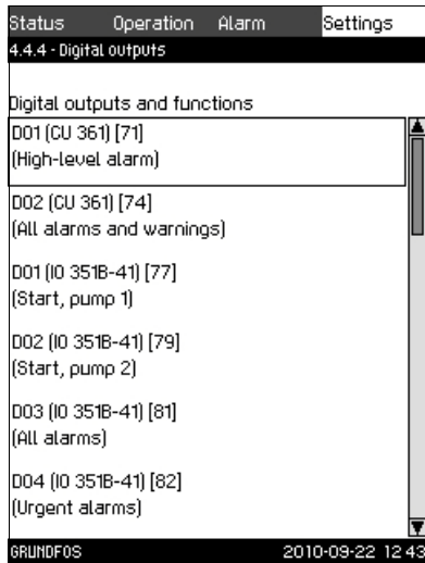
Fig. 30 Digital outputs
