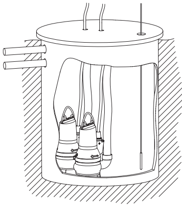
Fig. 17 Example of a two-pump installation (factory settings)
