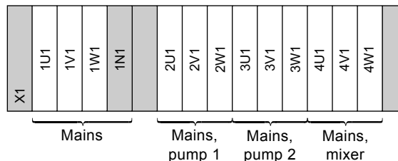
Fig. 3 Terminal block X1, mains supply
