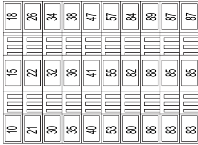
Fig. 5 Terminal block X3, IO 351B
