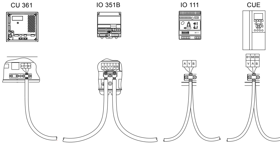
Fig. 15 GENIbus connection
