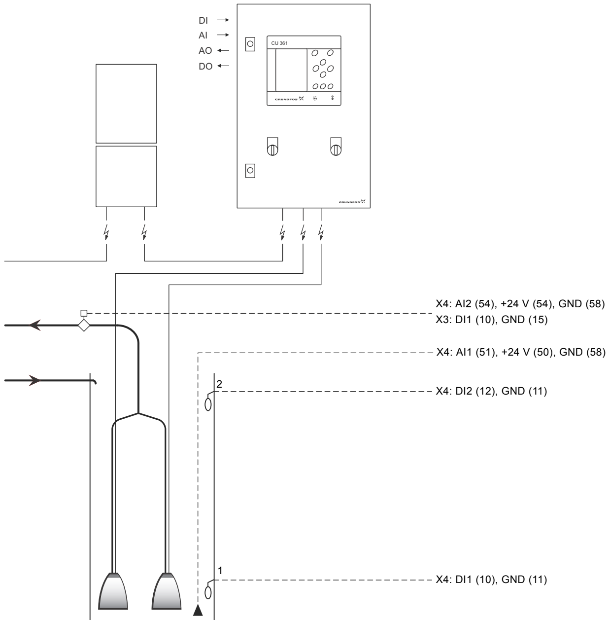
Fig. 8 Two pumps with analog level sensor and safety float switches
