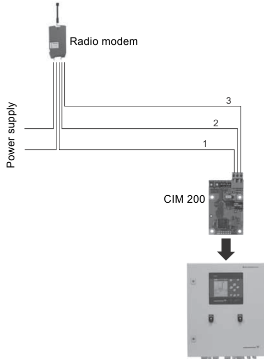
Fig. 22 Radio modem connection via Modbus RTU
